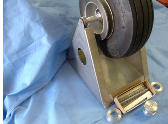
Tire Balance
