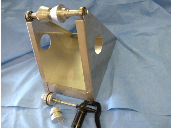
Bearing Greaser
